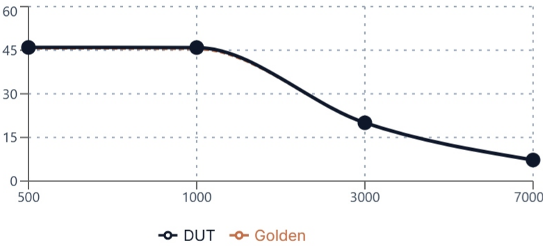
TORQUE vs SPEED (Nm)
