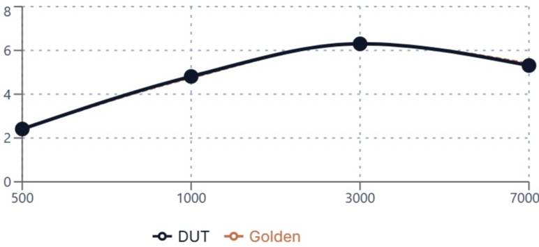
POWER vs SPEED (kW)
